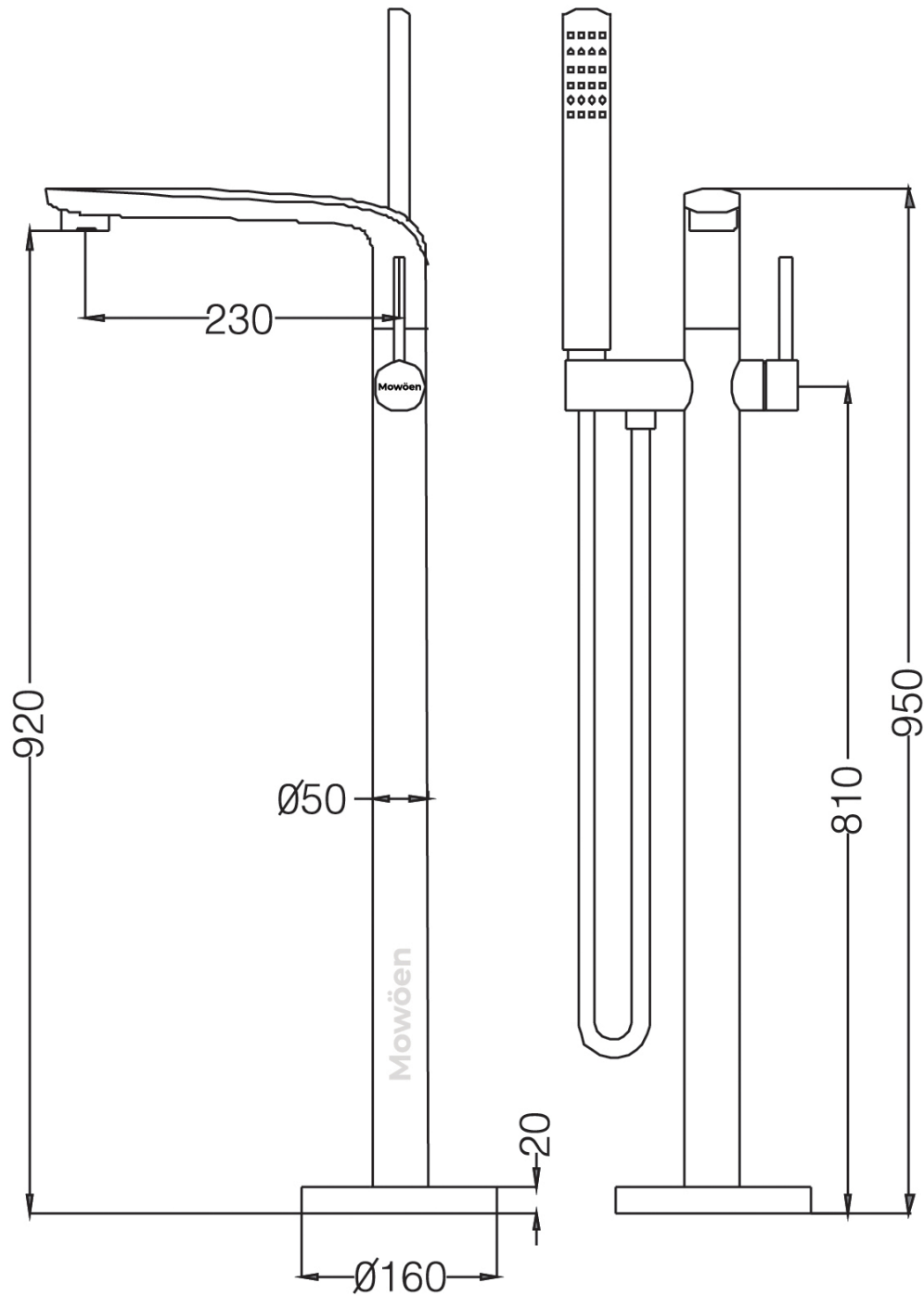
Side view
