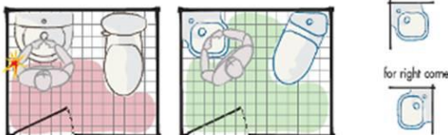
Wall Hung Basin (Corner) Size:450 x 405 x 180 mm.
