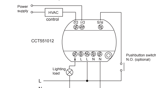
Fig 7. Wiring diagram for a typical dual load application
